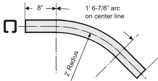
2'-0" RAD. 45° Upper Vertical Curve 20113
